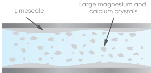
Large lime crystals in water make pipes narrower due to limescale
