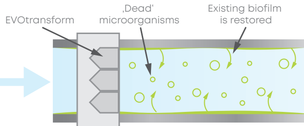
With less corrosion and limescale, no more 'dead' microorganisms can settle
